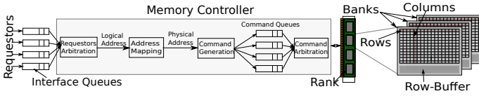
Fig. 1: DRAM subsystem.
