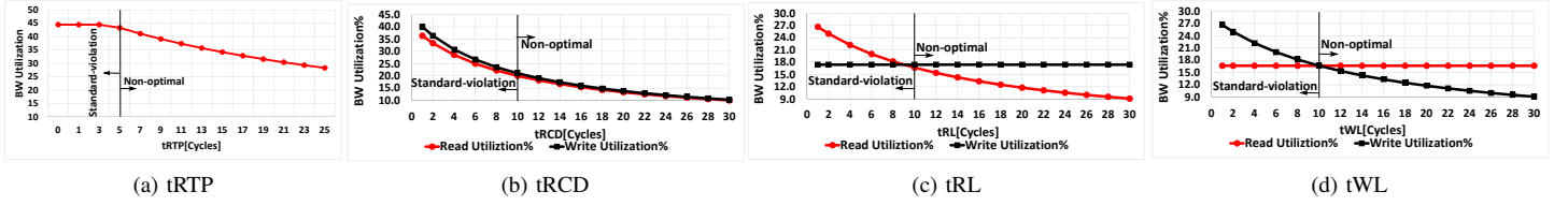
Fig. 7: Timing parameters validation.
